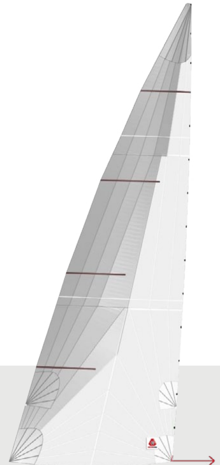
TRIRADIAL-CUT MODEL
